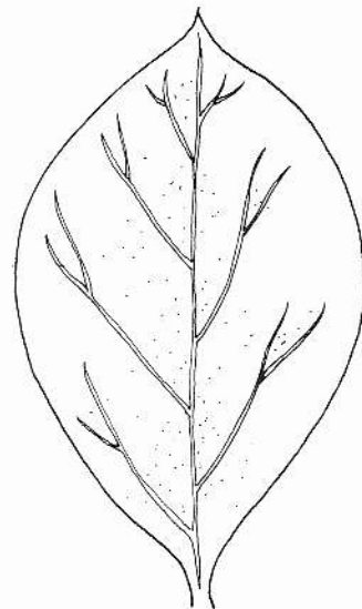
6 Obovate
